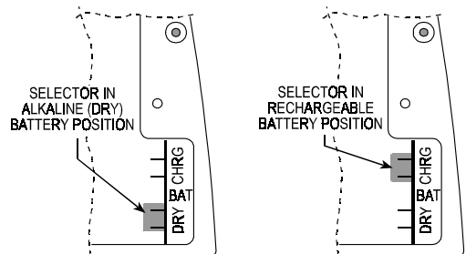
Figure 13. Battery Selector Positions
