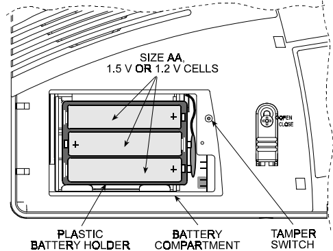
Figure 12. Battery Compartment and Battery Holder
